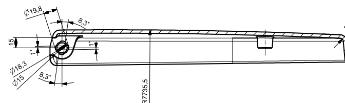
SECTION F-F
