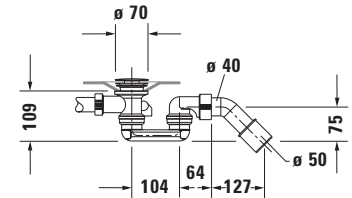
Siphon for bathtub # 700099
